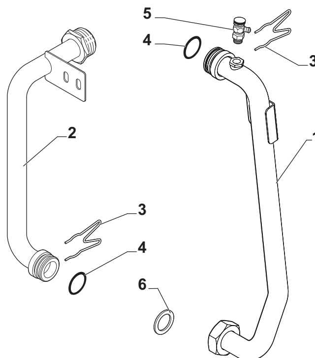
Fig.140 HC 2-19 FF / HC 2-24 FF / HC 2-32 FF
